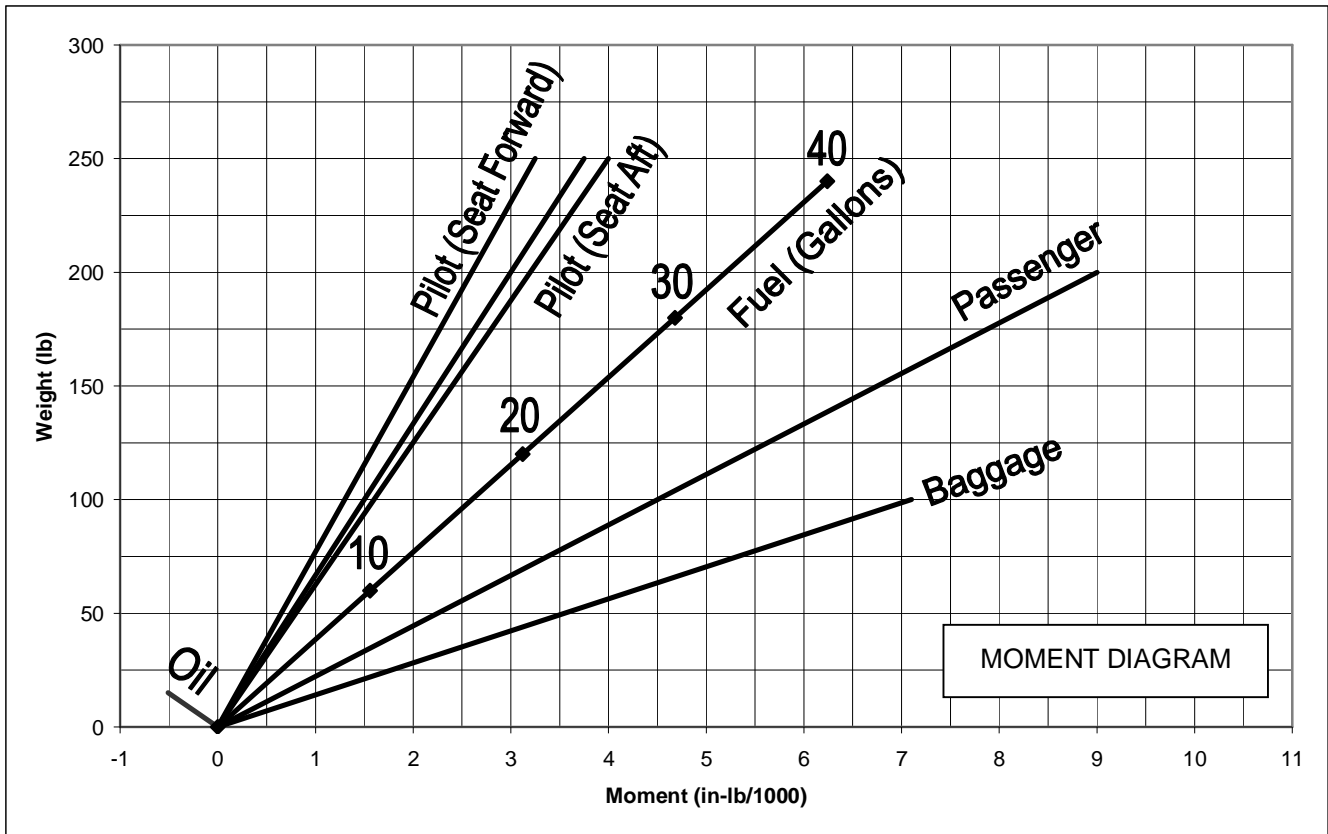
Figure 2, Revised Loading Chart
