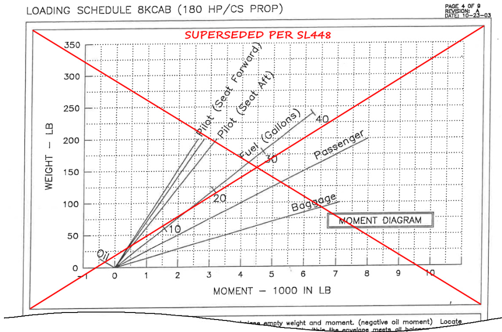
Figure 1, Superseded Loading Schedule
